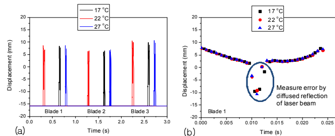
Figure 9. (a) Laser displacement sensor response at various temperatures, (b) Displacement comparison at different temperatures.
