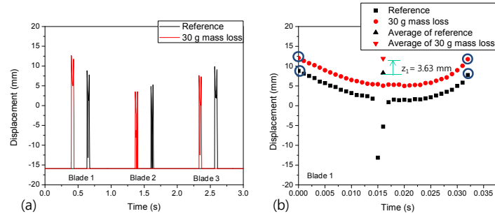
Figure 7. (a) Comparison of blade displacement variation in different blades before and after 30-g mass loss; (b) 30-g mass loss in Blade 1 resulted in -3.63-mm blade displacement.
