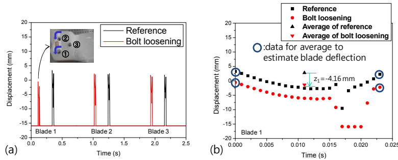
Figure 3. Bolt loosening monitoring at 100 mm from the blade tip: (a) Blade displacement before and after bolt loosening, (b) Comparison of displacements for Blade 1.
