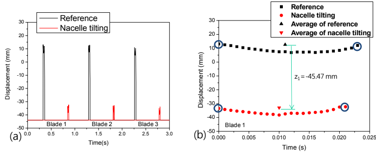
Figure 5. Nacelle tilts monitoring at 100 mm from the blade tip: (a) comparison of blade displacement before and after nacelle tilt and (b) variation in displacement of Blade 1 due to nacelle tilting.
