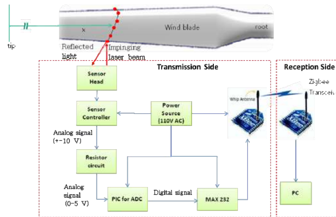
Figure 10. A block diagram showing the wireless module for remote monitoring.
