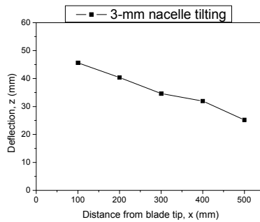
Figure 6. Comparisons of the variation in deflection due to the nacelle tilt at different distances from the blade tip.
