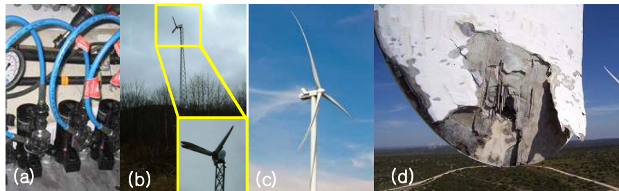
Figure 1. (a) Bolts used in wind turbine blades [3]. (b) Collision accident between the blade and the tower caused by nacelle tilt [4]. (c) Bent wind turbine blade with blade tip closer to the tower (V112-Vestas) [5]. (d) Lightning-induced blade tip damage [6].
