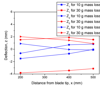
Figure 8. Deflection monitoring results at different mass loss and distances from the blade tip.
