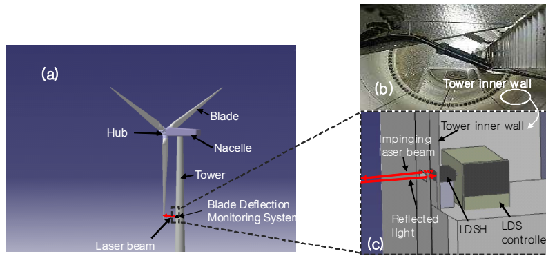
Figure 2. (a) Installation of the blade deflection monitoring system within the tower. (b) Inside the actual wind turbine tower. (c) Inside wind turbine tower with laser displacement sensor (LDS) installation.
