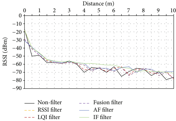
FIGURE 8: Smoothed RSSI values using all filters for half-open and half-closed space environment.
