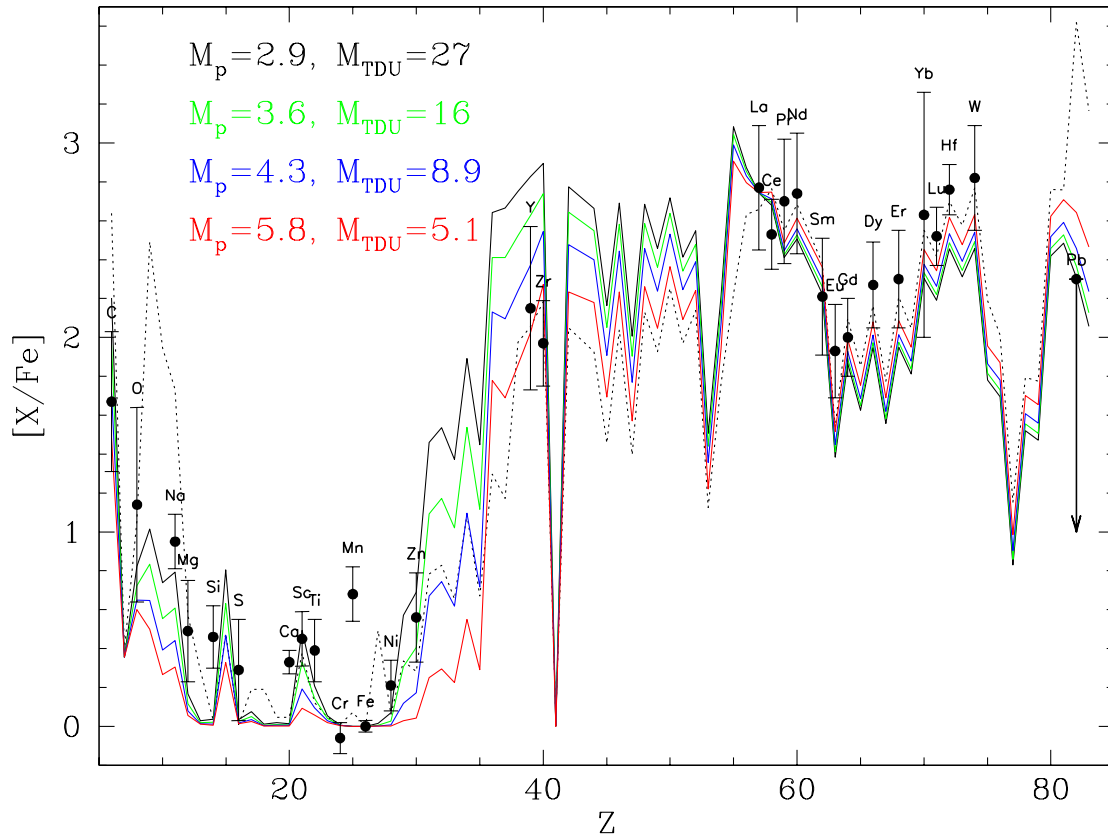
Figure 1. Comparison of AGB model predictions, computed on the basis of a stellar structure with initial 1.3 M_{\odot} and [\text{Fe}/\text{H}] = -1.3 , to the composition of the post-AGB star J004441.04-732136.4 [46]. The dotted black line represents the results obtained introducing a ^{13}\text{C} pocket resulting from the mixing an exponentially decreasing proton profile over a mass of 0.002 M_{\odot} and with a parametric TDU of 0.0096 M_{\odot} . The TDU is fixed to match the observed [\text{La}/\text{Fe}] ratio. The colored lines represent the results obtained by artificially ingesting in the third-last TP a mass of protons between 2.9 and 5.8 (in units of 10^{-6} M_{\odot} ), and with a parametric TDU between 5.1 and 27 (in units of 10^{-4} M_{\odot} ).
