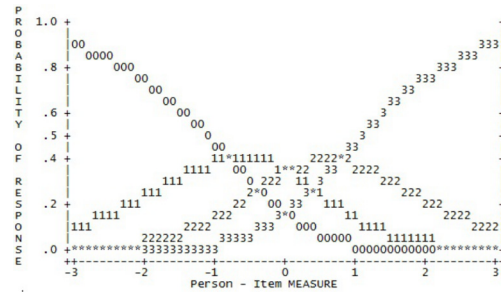
Fig 2. Response probability curve with collapsed 4-point response options (Factor 5).
