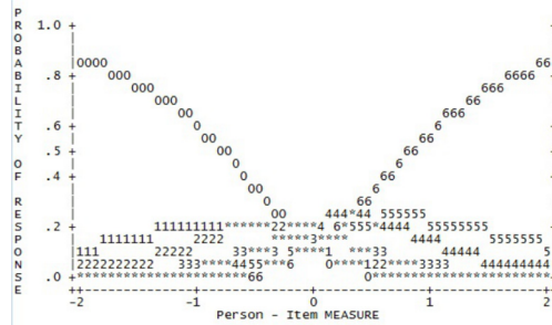
Fig 1. Response probability curve with original 7-point response options (Factor 5).
