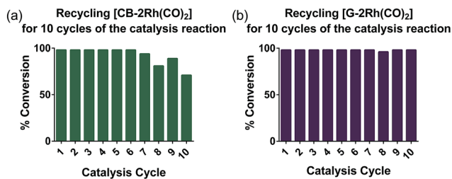
Fig. 6 Graphs depicting: (a) the % conversions of the hydrosilylation reaction for 10 reaction cycles when using [\text{CB-2Rh}(\text{CO})_2] and (b) the % conversions of the hydrosilylation reaction for 10 reaction cycles when using [\text{G-2Rh}(\text{CO})_2] .
