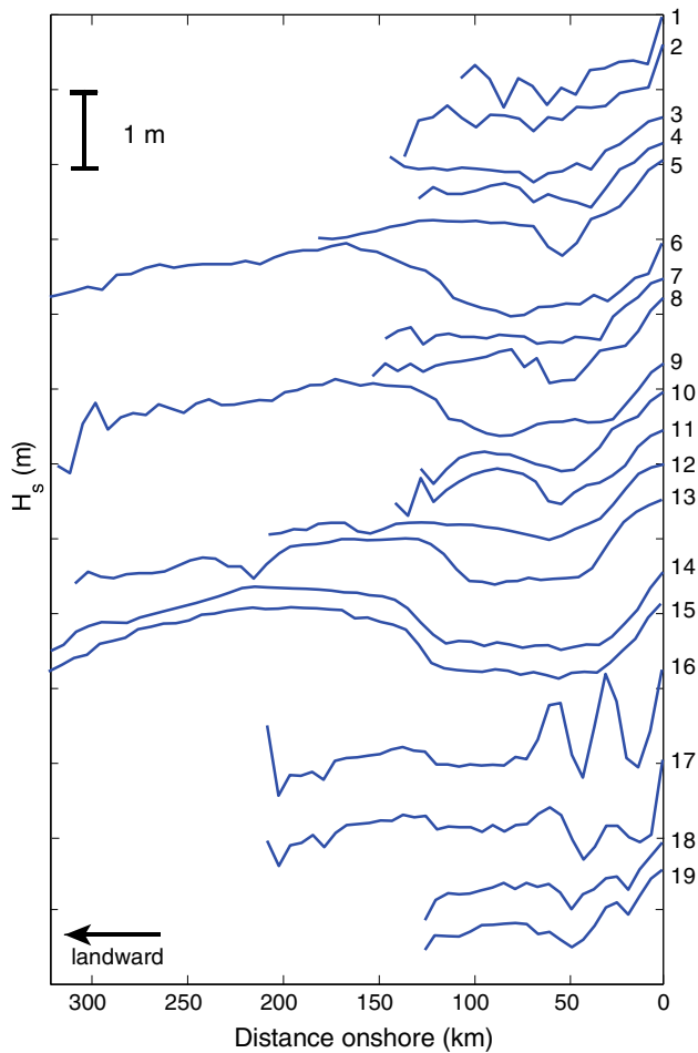
Fig. 10 Mean values of H_s along all tracks from north to south (top to bottom of plot). The track number is shown on the right. Distance onshore is from the offshore point seaward of the reef matrix for each altimeter pass
