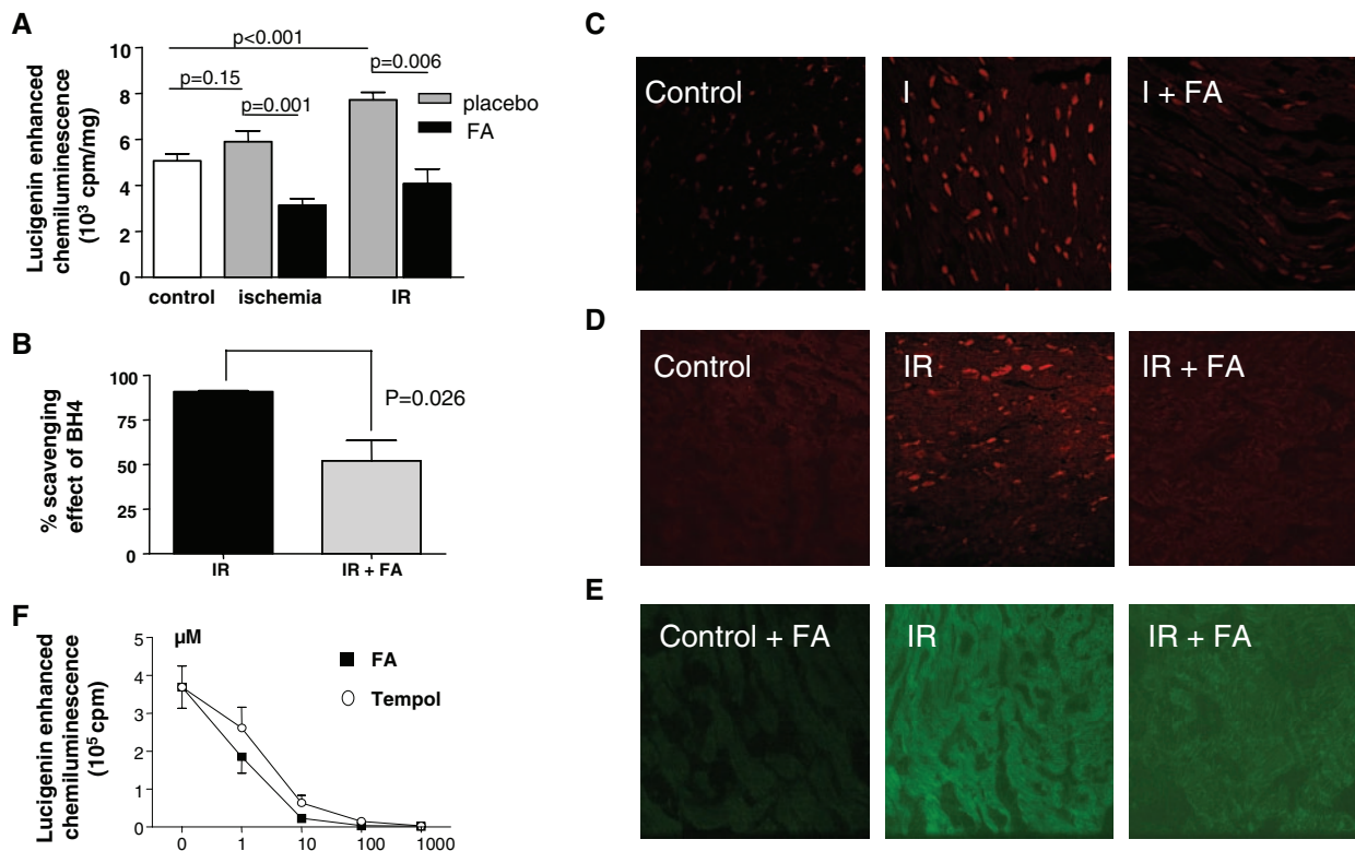
Figure 5. Effects of FA treatment on ROS generation. A , Lucigenin-enhanced superoxide detection shows marked reductions in ischemia and IR-induced superoxide with FA pretreatment. B , O_2^- formation in control vehicle-treated IR hearts was markedly suppressed by the acute addition of BH_4 , whereas it was blunted by nearly half in myocardial extracts obtained from FA-pretreated hearts. Dihydroethidium (DHE)-stained ( C , D ), and dichlorodihydrofluorescein diacetate (DCF)-stained ( E ) myocardia reveal increased ROS generation in ischemic or IR myocardium that was substantially reduced in heart receiving FA pretreatment. F , Direct antioxidant effects of FA compared with Tempol. Superoxide was generated by xanthine/xanthine oxidase in vitro and measured by lucigenin-enhanced chemiluminescence at various added concentrations of either FA or Tempol.
