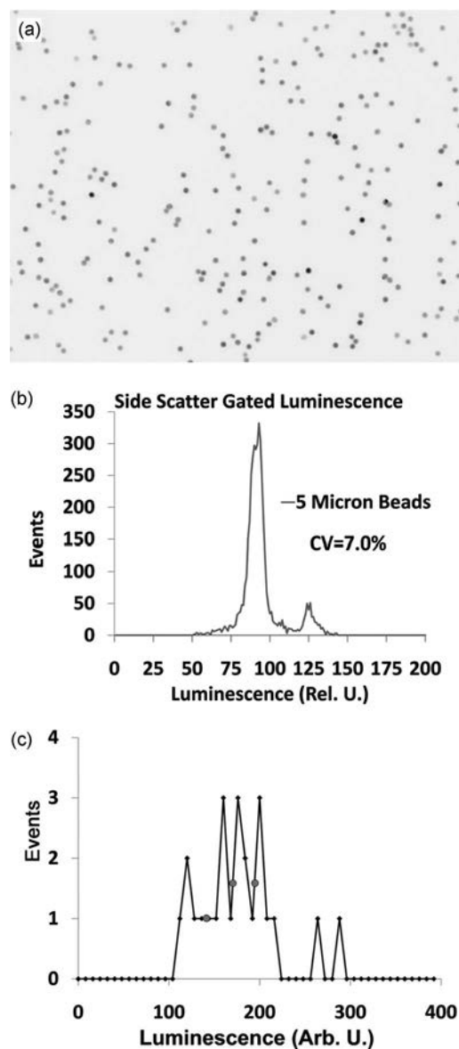
Fig. 3 Newport Instrument's Fire Red 5- \mu m europium-calibration beads. (a) Luminescence image obtained with a 10 \times 0.25 -NA objective with 2 \times 2 binning. The exposure was approximately 1 s. The 200-mw UV LED was used for excitation. The beads are essentially homogeneous except for a few dark ones. The image has been inverted. (b) Luminescence distribution obtained with light-scatter-gated flow cytometer. (c) Luminescence histogram obtained from an image of 24 beads. The three dots \bullet are located at 25, 50, and 75% of the area of the histogram.
