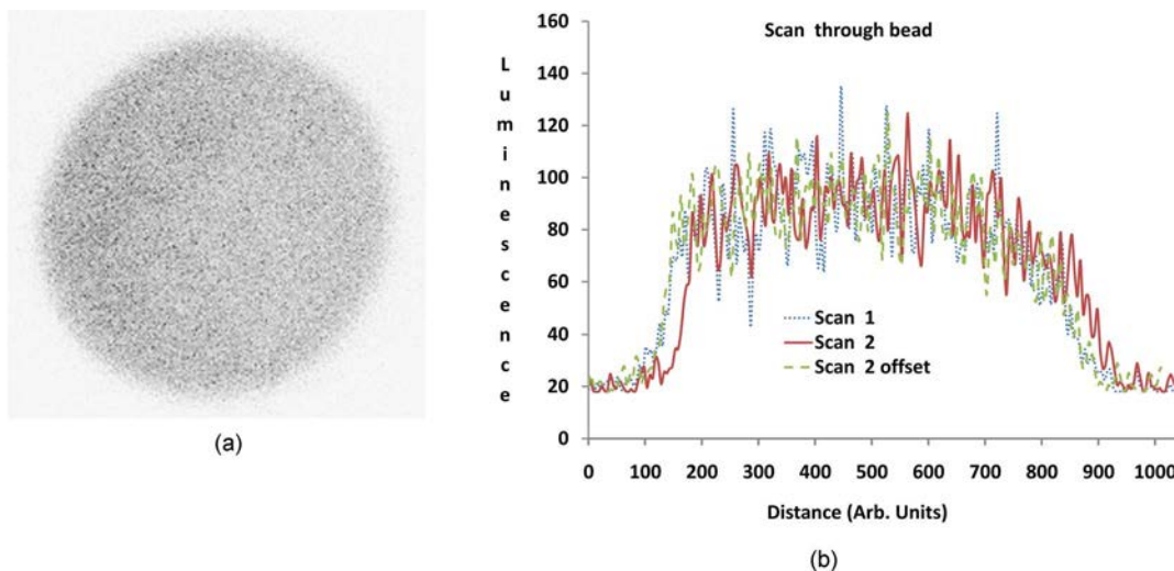
Fig. 5 (a) shows an inverted monochrome confocal image of the center section of a 5- \mu\text{m} bead and (b) shows two adjacent line scans of the luminescence (arbitrary units) through the center of the image. Scan 2 was offset to try to line it up with scan 1. (Color online only).
