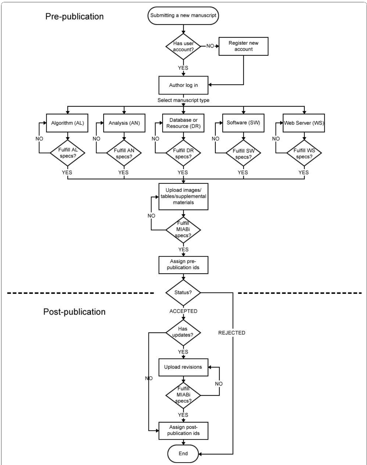
Figure 2 The MIABi workflow. Pre-publication and post-publications sections of the workflow are elaborated.
