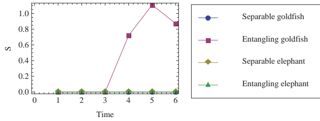
FIG. 6. (Color online) Spatial entanglement dynamics of 2D short-term-memory and long-term-memory quantum walks, with separable and entangling coins. We only observe spatial entanglement when the coin is entangling and there is no memory.
