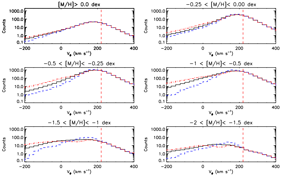
Figure 9. Azimuthal velocity histograms for different metallicity bins and for the stars being between 1 and 2 kpc above the Galactic plane. The counts are averaged on the total of the 500 Monte Carlo simulations. The black histograms represent the result obtained with the actual derived distances, whereas the blue and red ones are the results obtained with distances modified by -50 and +50 per cent, respectively, for the stars with V_\phi < 100 \text{ km s}^{-1} (which is an overestimation of the possible distance bias of 20 per cent for the giant stars; see Binney et al. 2013b). The vertical red dashed line is positioned at V_{\text{LSR}} = 220 \text{ km s}^{-1} .
