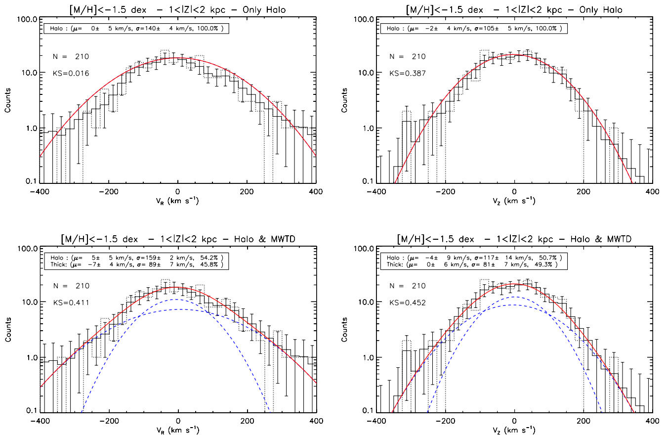
Figure 15. Radial (left) and vertical (right) orbital velocity distributions for all the stars with [M/H] < -1.5 dex being between 1 and 2 kpc far from the Galactic plane. The top panels show the fit when only one Galactic component, the halo, is used in order to fit the data, whereas the bottom panels consider two Gaussians (one for the thick disc and one for the halo).
