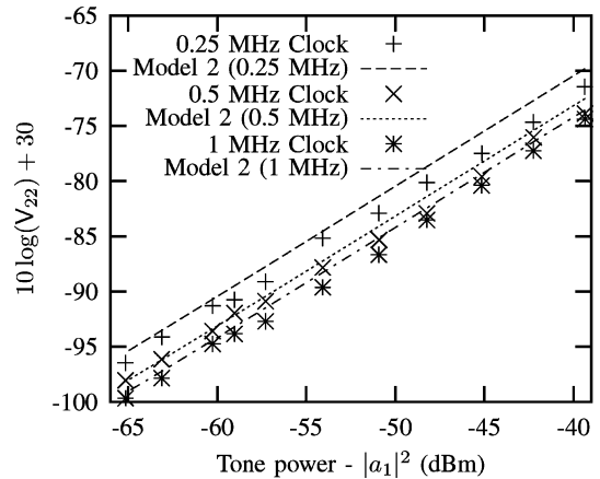
Fig. 11. Comparison of the sample variance V_{22} and the variance predicted by Covariance Model 2 for different phase reference clock frequencies. The instrument IF bandwidth was set to 100 Hz. The Agilent E4437 signal generator was used to drive the phase reference. For these measurements, the model is able to predict the change in variance for different phase reference clock frequencies (change in phase reference magnitude |R| ). Note that the clock frequency reported on the plot is approximate for clarity. 0.25-MHz clock is 0.24375 MHz, 0.5-MHz clock is 0.4875 MHz, and 1-MHz clock is 0.975 MHz.
