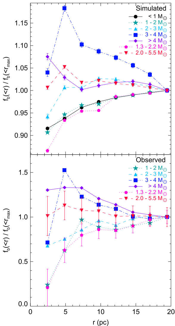
Figure 7. Comparison of the radial distributions of the binary frequency in different mass bins for one simulation of NGC 1818 with [Q, D] = [0.5, 2] from Geller et al. (2013b, top) and the observations from Li et al. (2013, bottom). The different plotting styles for the different mass bins are indicated on each plot. As in Figure 2, we show the binary frequency inside the given radius. We only count binaries with mass ratios q = m_2/m_1 \geq 0.55 , and any binary with q < 0.55 is counted as a single star. For the simulation, we use the same 1000 sight lines as in Geller et al. (2013b); the points in the top panel show the means of these values, with uncertainties (visible when larger than the plotted symbols) indicating the standard error on these means. Uncertainties on the observations (derived using Poisson counting statistics, see Li et al. 2013) are much larger, and are shown in the bottom panel for two representative samples for clarity.
