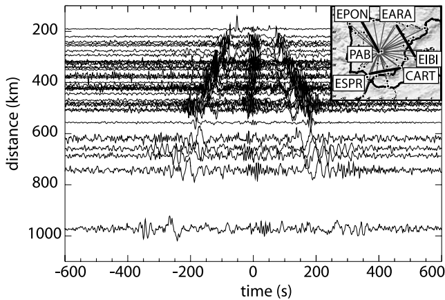
Figure 2. Record section of raw (unfiltered) cross correlations of stations in the Iberian Peninsula with respect to station PAB obtained using 4 months of ambient noise data. The causal (positive time) and acausal (negative time) arrivals of the Rayleigh wave are clearly visible in all records. The inset shows the location of the paths corresponding to the record section shown in this figure (thin gray lines) and of the group velocity measurements shown in Figure 3 (thick black lines).
