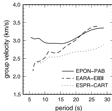
Figure 3. Example of group velocity measurements of fundamental-mode Rayleigh waves from ambient noise cross correlations for interstation paths sampling different structural units of the Iberian region (see Figure 2 for location). The station codes for the two stations that define each path are also indicated.
