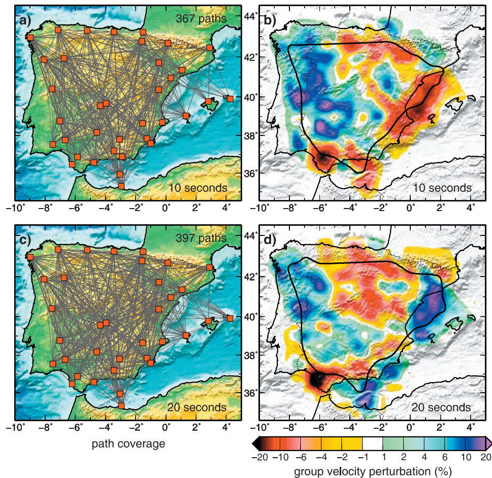
Figure 4. Ray path coverage and group velocity maps obtained for the 10 and 20 s period Rayleigh waves: (a) ray path coverage of 10 s group velocity Rayleigh wave measurements used in the tomographic inversion, (b) Rayleigh wave group velocity map at 10 s, (c) ray path coverage of 20 s group velocity Rayleigh wave measurements used in the tomographic inversion, and Rayleigh wave group velocity map at 20 s (Figure 4b). Within the thick contour line (drawn in Figures 4b and 4d), features wider than 100 km are well resolved.
