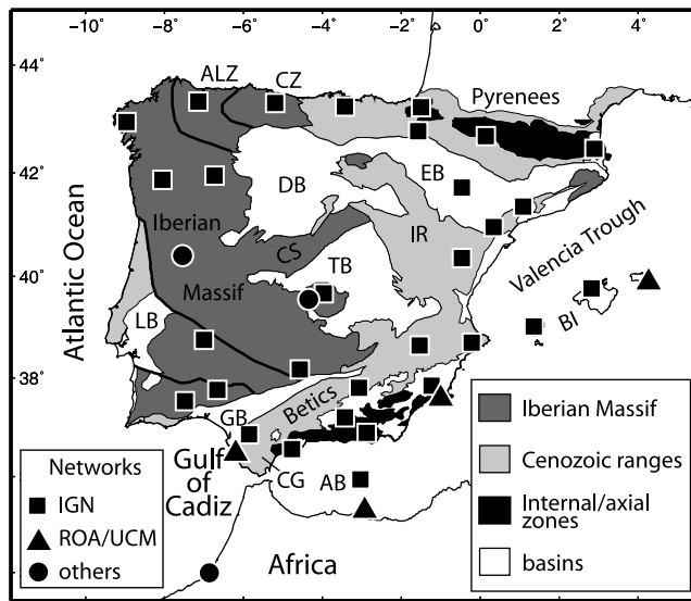
Figure 1. Structural map of the Iberian Peninsula, showing the major sedimentary basins and the location of the seismic stations used in this study (modified from Vergés and Fernández [2006]). Different station symbols indicate network affiliation and are explained in the inset. AB, Alboran Basin; ALZ, Astur-Leonese Zone; BI, Balearic Islands; CG, Campo de Gibraltar flysch units; CS, Central System; CZ, Cantabrian Zone; DB, Duero Basin; EB, Ebro Basin; GB, Guadalquivir Basin; IR, Iberian Range; LB, Lusitanian Basin; TB, Tagus Basin.
