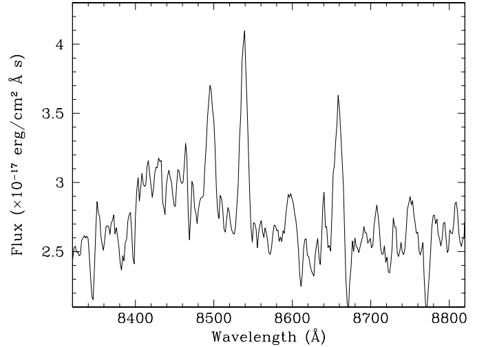
Fig. 6. CaII 8498, 8542 and 8662 Å emission lines at the central star. The nebulal spectrum has been subtracted. The Pa14 and Pa12 HI lines at 8598 Å and 8750 Å, respectively, are barely detected.
