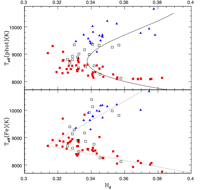
Fig. 6. Upper panel: comparison between temperatures from photometry ( T_{\text{eff}}(\text{Phot}) ) and the index of the strength of the H_{\delta} line ( H_{\delta} ); over-imposed is the relation expected from theoretical models (see Munari et al. 2005). Lower panel: the same, but for temperatures from Fe lines ( T_{\text{eff}}(\text{Fe}) ). Different symbols are for stars of different groups (see Sect. 4): Group 1: red filled squares; Group 2: black open squares; Group 3: blue filled triangles. The fit lines used to define T_{\text{Cool}} and T_{\text{Hot}} are also plotted in the bottom panel .
