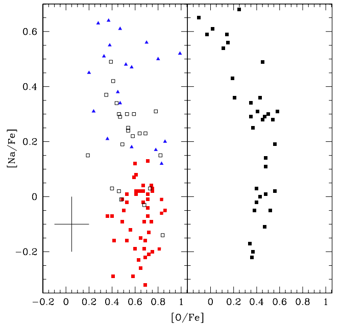
Fig. 18. [O/Fe] vs. [Na/Fe] for BHB stars ( left panel ) and RGB stars from Marino et al. (2011a: right panel ). In the left panel different colours are for stars of different groups (see Sect. 4). Group 1: red filled squares; Group 2: black open squares; Group 3: blue filled triangles. Typical error bars for our analysis are also shown.
