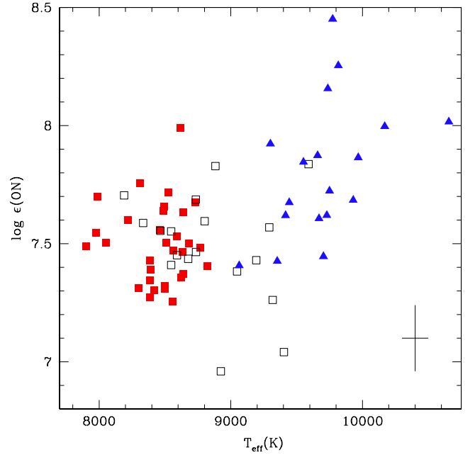
Fig. 17. T_{\text{eff}} vs. the sum of N and O abundances. Different colours are for stars of different groups (see Sect. 4). Group 1: red filled squares; Group 2: black open squares; Group 3: blue filled triangles.
