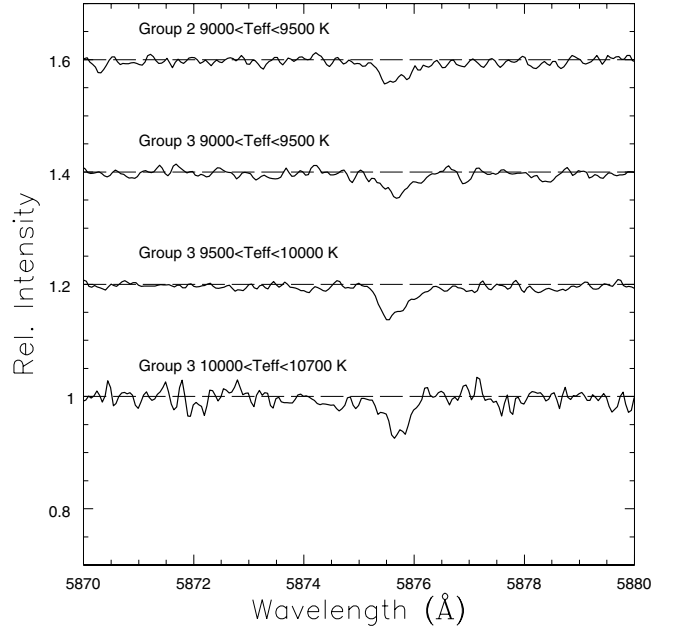
Fig. 11. Average spectra in the region of the He I line at 5876 Å for stars in different temperature bins. See Sect. 4 for the definition of different groups of stars. Spectra have been offset for clarity.
