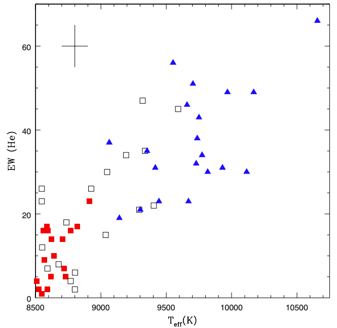
Fig. 12. T_{\text{eff}} vs. the equivalent width of the He I line at 5876 Å. Different colours are for stars of different groups (see Sect. 4): Group 1: red filled squares; Group 2: black open squares; Group 3: blue filled triangles. Typical error bars are also shown.
