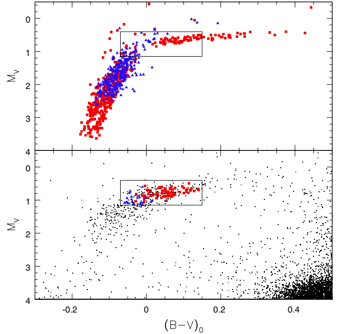
Fig. 20. Comparison between a synthetic ( upper panel ) and an observed ( lower panel ) colour-magnitude diagram for the horizontal branch of M22. Red squares are metal-poor stars (in the lower panel , stars of Groups 1 and 2); blue triangles are metal-rich stars (in the lower panel , stars of Group 3). In the lower panel , stars not observed in this paper are dots. The region of the HB observed in this paper is marked with a rectangle in both panels.
