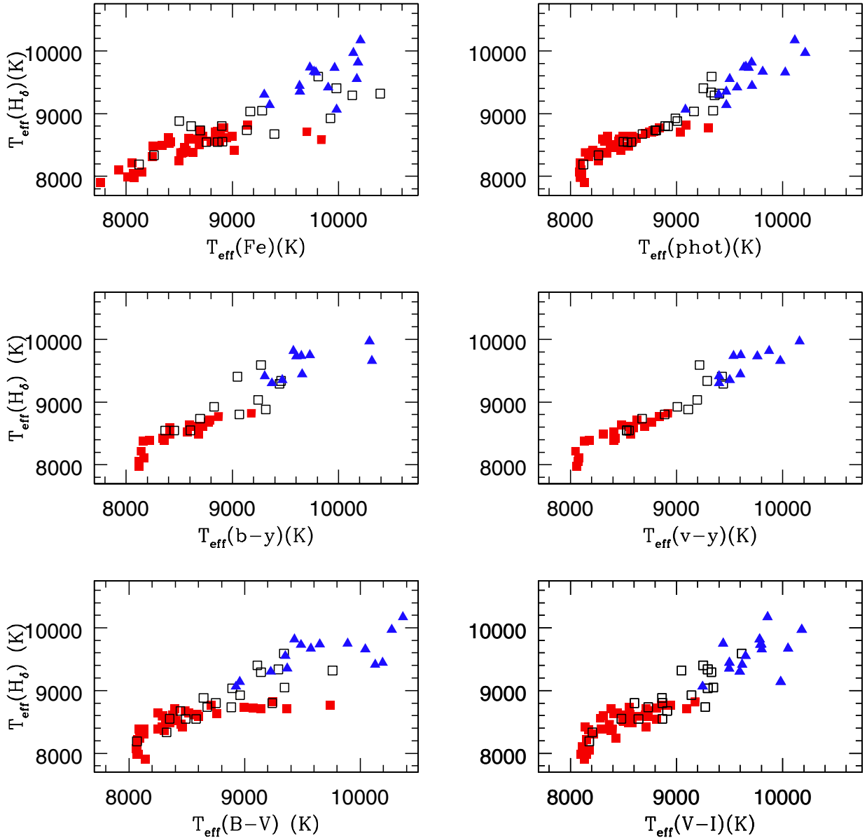
Fig. 8. Comparison between temperatures from colours and their average ( T_{\text{eff}}(\text{phot}) ) and from our calibration of the H \delta line ( T_{\text{eff}}(\text{H}\delta) ). Different colours are for stars of different groups (see Sect. 4). Group 1: red filled squares; Group 2: black open squares; Group 3: blue filled triangles.
