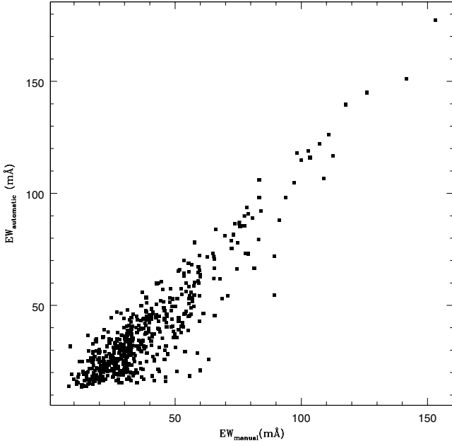
Fig. 9. Comparison between EWs measured manually and by the automatic procedure described in the text. The automatic EWs were corrected for the relation given in the text before being plotted.
