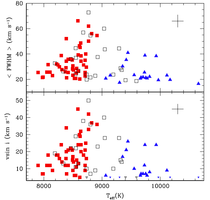
Fig. 4. T_{\text{eff}} vs. FWHM of lines ( upper panel ) and rotational velocity ( v \sin i ; lower panel ); different colours are for stars of different groups (see Sect. 4): Group 1: red filled squares; Group 2: black open squares; Group 3: blue filled triangles. Small triangles in the lower panel represent upper limits in v \sin i . Typical error bars are also shown.
