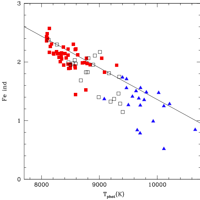
Fig. 7. Comparison between the Fe I line strength index Fe-Ind and temperatures from photometry ( T_{\text{eff}}(\text{Phot}) ). Different symbols are for stars of different groups (see Sect. 4): Group 1: red filled squares; Group 2: black open squares; Group 3: blue filled triangles. Superimposed is the calibration line we used.
