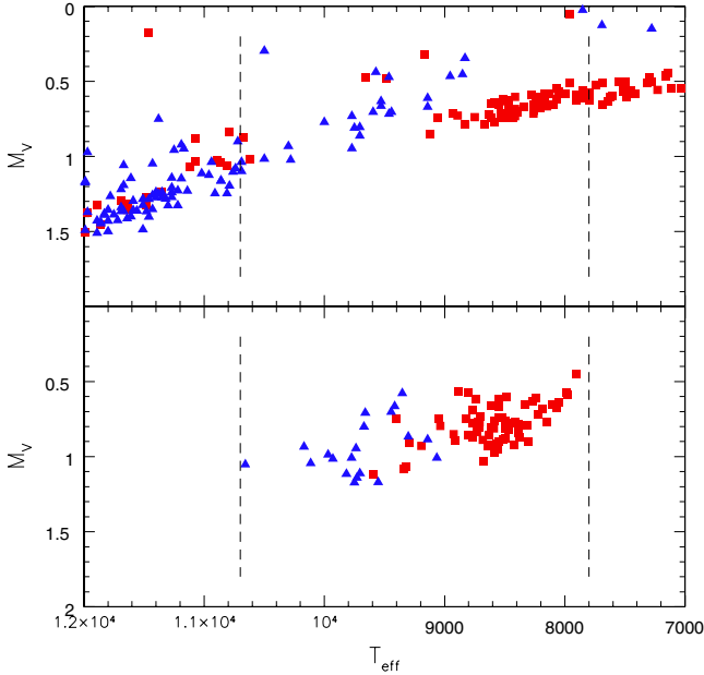
Fig. 21. Details of the comparison between synthetic ( upper panel ) and observed ( lower panel ) T_{\text{eff}} - M_V diagram for the horizontal branch of M 22. Red squares are metal-poor stars (in the lower panel , stars of groups 1 and 2); blue triangles are metal-rich stars (in the lower panel , stars of group 3). The region of the HB observed in this paper is within the dashed lines in both panels .
