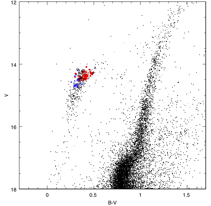
Fig. 1. (V, B - V) colour–magnitude diagram of M 22 from Monaco et al. (2004). Different symbols are for stars of different groups (see Sect. 4): Group 1: red filled squares; Group 2: black open squares; Group 3: blue filled triangles. Dots are the stars not observed in this paper.
