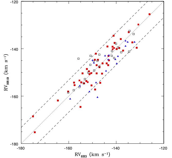
Fig. 2. Radial velocities from set-up HR03 vs. those from set-up HR19A; different colours are for stars of different groups (see Sect. 4): Group 1: red filled squares; Group 2: black open squares; Group 3: blue filled triangles. Dotted line represents equality; dashed lines are \pm 2 times the observational errors.
