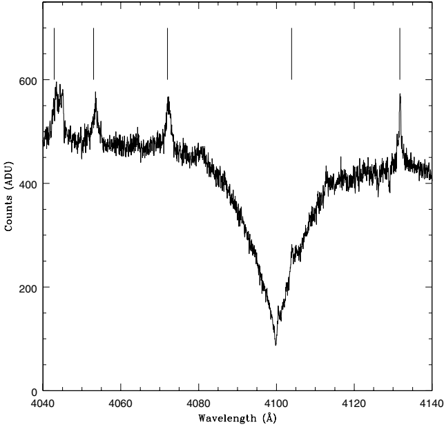
Fig. 5. Portion of the spectrum of star 115 including H_{\delta} . This is the most extreme case of stronger contamination by Th-Ar lines. Identification of several contaminating lines is from the Kitt Peak Th-Ar spectrum ( http://old-www.noao.edu/kpno/specatlas/thar/ ).
