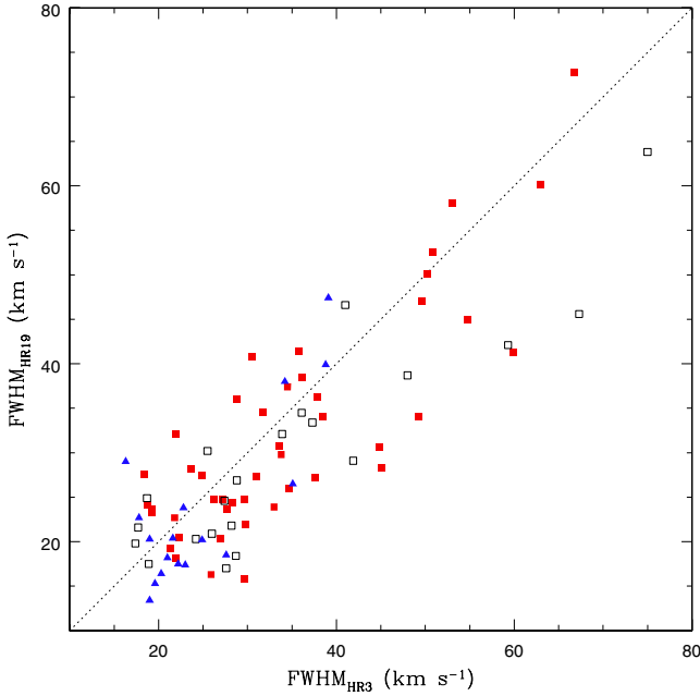
Fig. 3. FWHM of lines from set up HR03 vs. those from set up HR19A; different colours are for stars of different groups (see Sect. 4): Group 1: red filled squares; Group 2: black open squares; Group 3: blue filled triangles.
