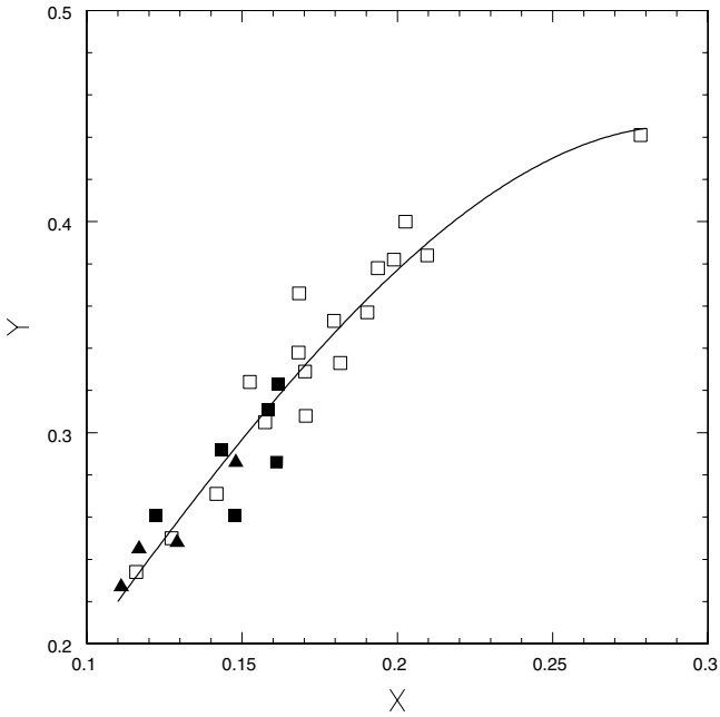
Fig. 13. Relation between the X index for the strength of the He I line at 5876 Å (see Eq. (2) for a definition) and the He abundance by mass Y for BHB stars in NGC 2808 (Marino et al. 2014: open squares), NGC 6752 (Villanova et al. 2009: filled triangles), and M 4 (Villanova et al. 2012: filled squares). He abundances from these two last papers were corrected for departures from LTE and a zero point offset of 0.036 in Y . Overimposed is the best fit cubic through the origin (Eq. (3)).
