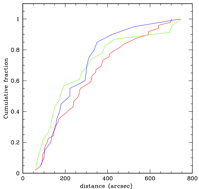
Fig. 19. Cumulative distribution of stars in different groups with separation from cluster centre. Different colours are for stars of different groups (see Sect. 4): Group 1: red; Group 2: green; Group 3: blue.
