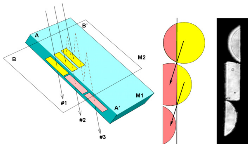
Figure 2. The Bowen-Walraven type image slicer. The resulting slices from a prototype are shown on the right.
