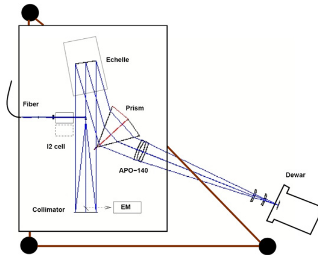
Figure 1. Optical and mechanical layout of the spectrometer. The rectangle outlines a standard optical table of 1 \times 1.5 m. A small mirror in front of the collimator deviates 1% of the light to the exposure meter.
