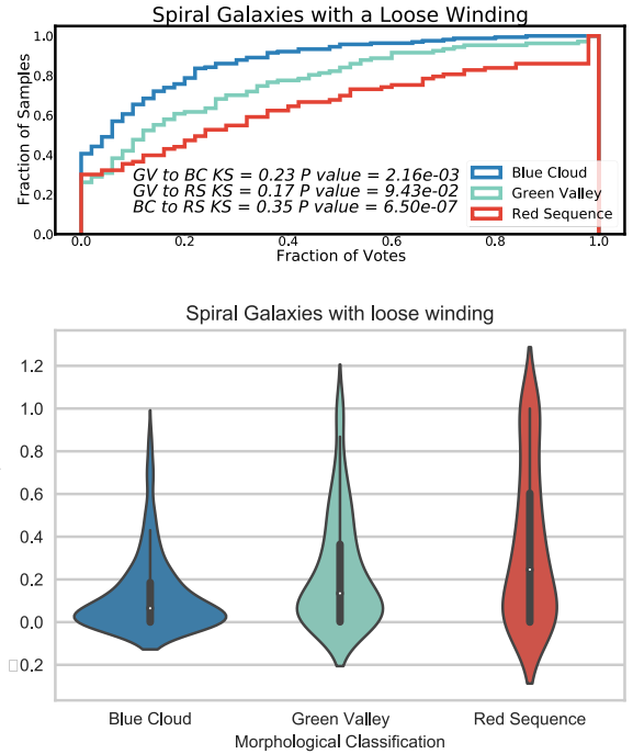
Figure 7. Histogram of the fraction of votes in favour of spiral galaxies having a loose winding (T05 in the GZ questionnaire). The difference between green-valley and blue-cloud galaxies is distinguishable with a KS of 0.23, the KS of green-valley and red-sequence galaxies is 0.17, and the KS of the blue cloud and red sequence is 0.35. Green valley to blue cloud has a p value of 2.16 \times 10^{-03} , green valley and red sequence is 9.43 \times 10^{-02} , and the KS of red sequence and blue cloud is 6.5 \times 10^{-07} . The violin plots in the lower panel represent the same data as the cumulative histogram at the top.
