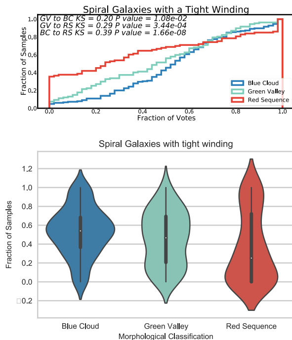
Figure 9. Histogram of the fraction of votes in favour of spiral galaxies having a tight winding (T05 in the GZ questionnaire). The difference between the green valley and blue cloud is distinguishable with a KS of 0.20, but the difference between the green valley and red sequence is 0.29, with the difference between the red sequence and blue cloud being the most distinguishable at 0.39. The significances of these are represented with p -values of the green valley and blue cloud of 1.08 \times 10^{-02} , green valley and red sequence of 3.44 \times 10^{-04} , and blue cloud and red sequence of 1.66 \times 10^{-08} . The violin plots represent the same data as the top panel histograms.
