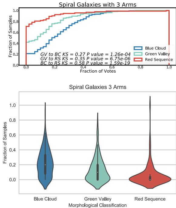
Figure 10. A histogram of the fraction of votes in favour of classifying galaxies as spiral with three arms (T10 in the GZ questionnaire). The difference between the green valley and blue cloud is very distinguishable with a K–S value of 0.27, green valley to red sequence is distinguishable with a K–S value of 0.35, and the highest difference is seen between blue cloud and red sequence with a K–S of 0.58. The significance from p -values is 1.26 \times 10^{-04} , 6.75 \times 10^{-06} , and 1.59 \times 10^{-19} , respectively. This shows that spiral galaxies with three arms are found more frequently in the blue cloud and green valley. The violin plots represent the same data.
