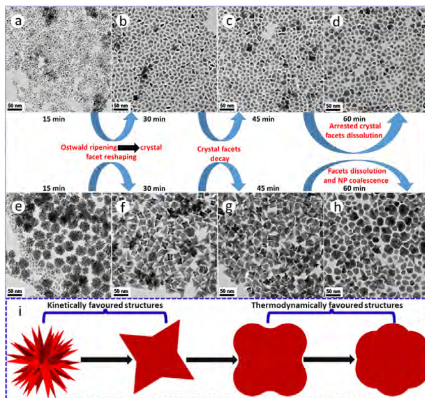
Figure 5. TEM BF images demonstrating the morphological transformations/changes of (a–d) PtNi and (e–h) Pt(NiCo) alloy NPs prepared by co-thermolytic decomposition of Pt and M (Ni and Co) acetylacetonate precursors. The colloidal alloy NP aliquots extracted from the bulk organic growth-mixture were sampled at different time intervals (from 15–60 min). (i) A corresponding schematic of geometrical restructuring from kinetically (high energy surface) to thermodynamically favourable (low energy surface) morphologies with extended ripening periods.
