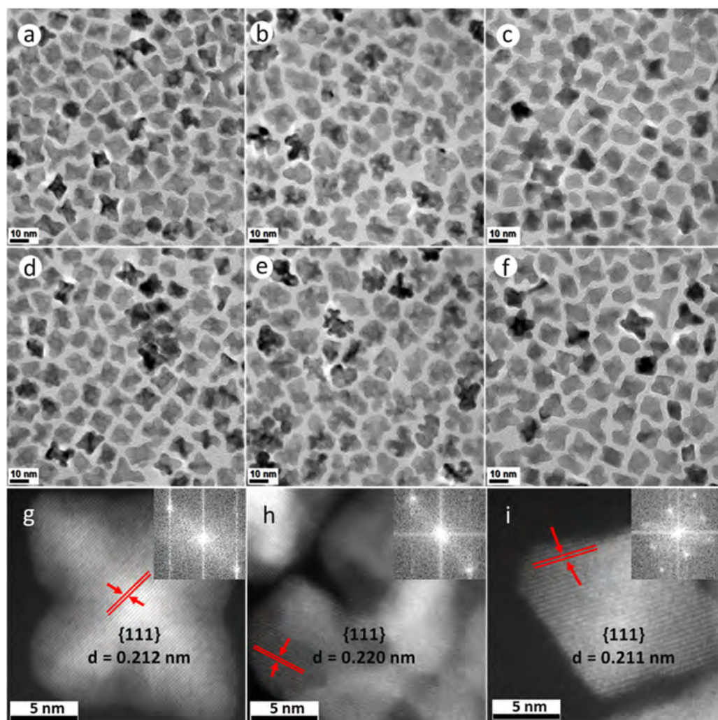
Figure 1. TEM bright field (BF) images of (a–f) PtNi, PtCo and Pt(NiCo) alloy NPs show insignificant morphological and size changes after the first measurement interval of 15 min (a–c) and the last 60 min (d–f). (g,h) Atomic-scale HAADF-STEM images of (g) PtNi, (h) PtCo and (i) Pt(NiCo) alloy NPs with good crystallinity and well-resolved lattice fringes confirming individual particles as perfect single crystals (insets are the assigned major facets, the calculated lattice spacings and FFT diffractograms).
