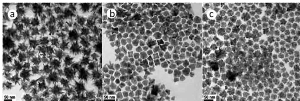
Figure 4. TEM BF images of PtNi, PtCo and Pt(NiCo) alloy NPs solution-grown via thermolytic decomposition of \text{Pt}(\text{acac})_2 in the presence of (a) \text{Ni}(\text{Ac})_2 , (b) \text{Co}(\text{Ac})_2 and (c) \text{Ni}(\text{Ac})_2 + \text{Co}(\text{Ac})_2 in dual amine surfactants OAm and HDA.
