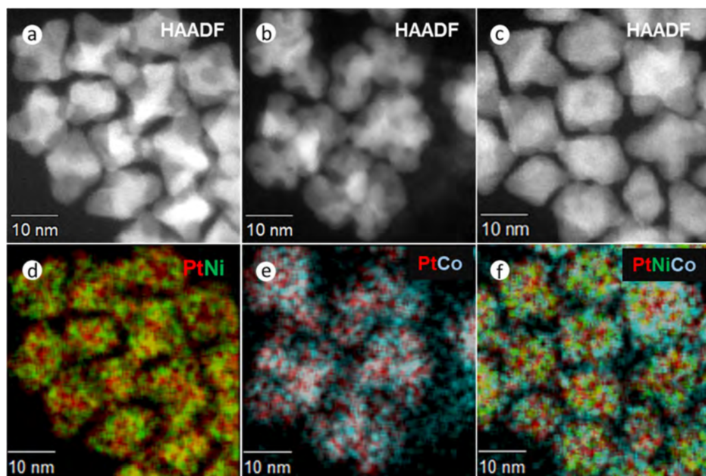
Figure 2. HAADF and STEM-EDS elemental distribution examination of PtNi, PtCo and Pt(NiCo) alloy NPs synthesized by Synthesis Method (a) (i). HAADF images of (a) PtNi, (b) PtCo and (c) Pt(NiCo) alloy NPs. (d–f) Composite EDX spectroscopic mappings of Ni ( K\alpha , green), Co ( K\alpha , cyan), and Pt ( L\alpha , red) reveal inhomogeneous distributions of two solid solutions (Pt-rich and M-rich phases) within the alloy NPs.
