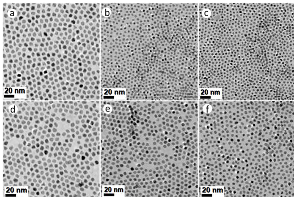
Figure 3. TEM BF images of PtNi, PtCo and Pt(NiCo) alloy NPs synthesized via simultaneous reduction of Pt(acac) 2 and non-noble organometallic precursors: (a) Ni(Ac) 2 , (b) Co(Ac) 2 and (c) Ni(Ac) 2 + Co(Ac) 2 ; (d) Ni(acac) 2 , (e) Co(acac) 2 and (f) Ni(acac) 2 + Co(acac) 2 in the presence pure amine surfactant OAm using the reductant Mo(CO) 6 . All the corresponding PXRD lines of these PtNi, PtCo and Pt(NiCo) alloy NPs displayed single solid solution phases.
