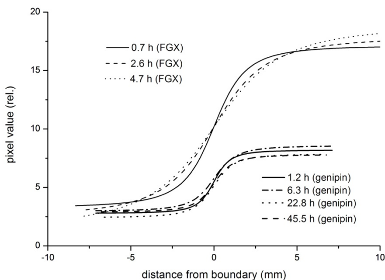
Figure 1. Fitted curves of image profiles of FGX gel (upper curves) and genipin-gelatin gel (lower curves) obtained at various times.
