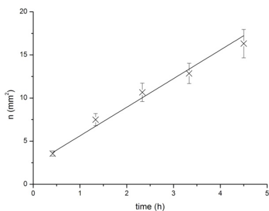
Figure 2a. The diffusion coefficient in this FGX gel was calculated from the slope of the linear fit of n versus time and was 0.70 \pm 0.05 \text{ mm}^2 \text{ h}^{-1} at 5 Gy.
