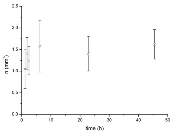
Figure 2b. The curvature parameter, n , did not significantly change over time for the genipin-gelatin gel dosimeter. Plotted are the average values (error bars indicate one standard deviation) of measurements of three samples from the same batch of gel.
