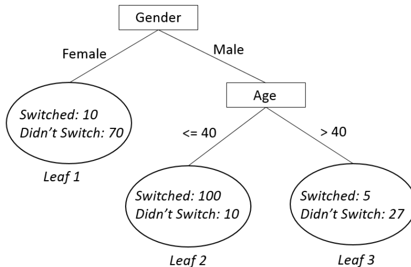
Figure 1: Example of a decision tree.
