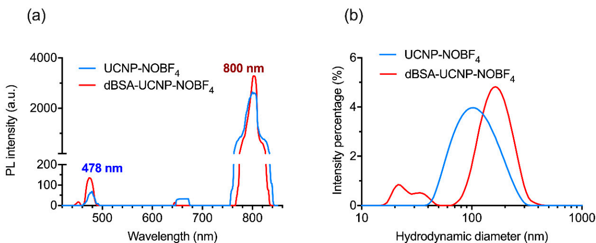
Figure 5. Characterization of UCNP-NOBF 4 and lyophilized dBSA-UCNP-NOBF 4 (dBSA at optimal concentration—10 μM): (a) PL emission spectrum of UCNP-NOBF 4 and lyophilized dBSA-UCNP-NOBF 4 under excitation at 980 nm; (b) hydrodynamic diameter distributions of UCNP-NOBF 4 and lyophilized dBSA-UCNP-NOBF 4 acquired by DLS in deionized water.
