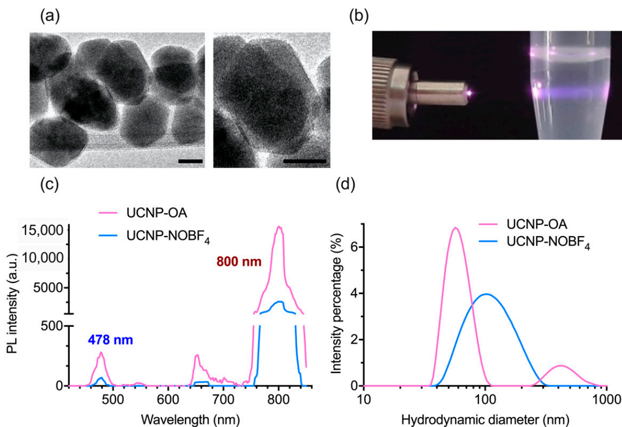
Figure 2. Characterization of UCNP-OA core/shell structure ( \text{NaY}_{0.794}\text{F}_4: \text{Yb}_{0.2}, \text{Tm}_{0.06}/\text{NaYF}_4 ) and UCNP-NOBF 4 : (a) TEM image of UCNP-OA, scale bar 20 nm; (b) UCNP in suspension illuminated by a laser with a wavelength of 980 nm; (c) photoluminescence (PL) emission spectrum of UCNP-OA and UCNP-NOBF 4 under excitation at 980 nm; (d) hydrodynamic diameter distributions of UCNP-OA and UCNP-NOBF 4 acquired by DLS in hexane and deionized water, respectively.
