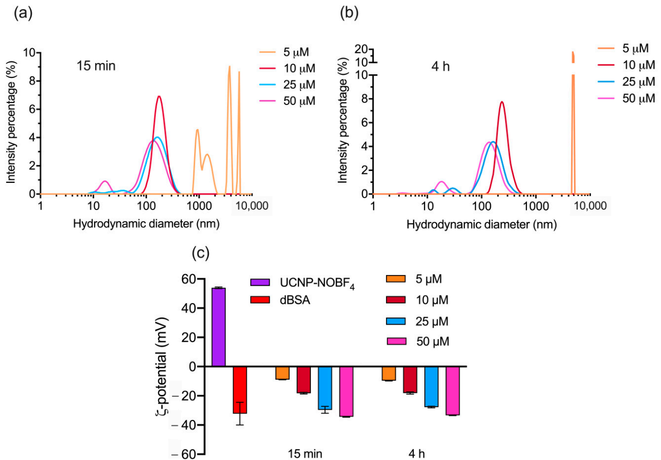
Figure 3. Concentration optimization of dBSA for forming PC on the surface of UCNP-NOBF 4 : (a,b) hydrodynamic diameter of dBSA-UCNP-NOBF 4 following the incubation of UCNP-NOBF 4 (0.25 mg/mL) with dBSA at different concentrations (5–50 μM) at room temperature for 15 min and 4 h, respectively measured by DLS; (c) the ζ-potential of UCNP-NOBF 4 , dBSA, and dBSA-UCNP-NOBF 4 recorded by electrophoretic light scattering (ELS). All samples were dispersed in deionized water.
