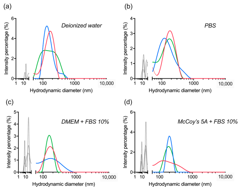
Figure 8. Evaluation of colloidal stability of lyophilized dBSA-UCNP-NOBF 4 in different buffers after one year of lyophilization and mixed by vortexing only, based on the results of three repeated size measurements (shown in blue, red, and green) by DLS: (a) in deionized water; (b) in PBS; (c) in DMEM cell culture medium supplemented with 10% FBS; (d) in McCoy's 5A cell culture medium supplemented with 10% fetal bovine serum (FBS). Gray and/or dotted lines below 100 nm correspond to the presence of proteins and protein aggregates; dotted lines over 300 nm are aggregates.
