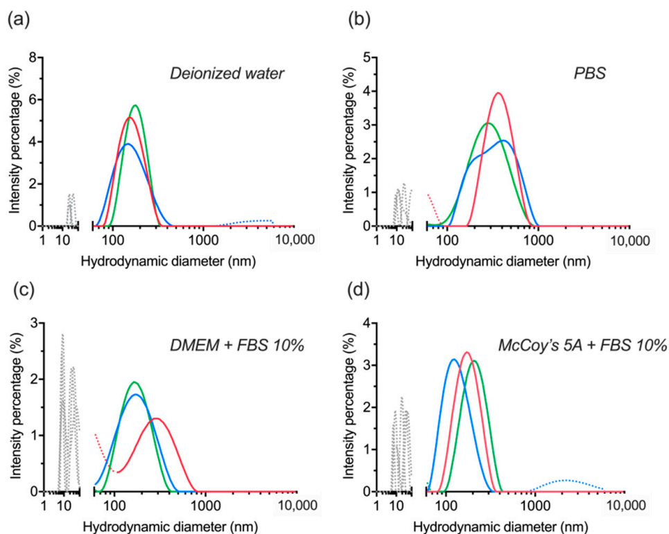
Figure 6. Evaluation of colloidal stability of lyophilized dBSA-UCNP-NOBF 4 in different buffers after one week of lyophilization and mixed by vortexing and ultrasonication, based on the results of three repeated size measurements (shown in blue, red, and green) by DLS: (a) in deionized water; (b) in PBS; (c) in DMEM cell culture medium supplemented with 10% FBS; (d) in McCoy's 5A cell culture medium supplemented with 10% FBS. Gray and/or dotted lines below 100 nm correspond to the presence of proteins and protein aggregates; dotted lines over 300 nm are aggregates.
