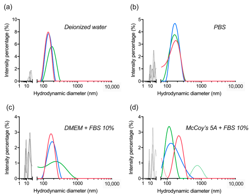
Figure 9. Evaluation of colloidal stability of lyophilized dBSA-UCNP-NOBF 4 in different buffers after one year of lyophilization and mixed by vortexing and ultrasonication, based on the results of three repeated size measurements (shown in blue, red, and green) by DLS: (a) in deionized water; (b) in PBS; (c) in DMEM cell culture medium supplemented with 10% FBS; (d) in McCoy's 5A cell culture medium supplemented with 10% FBS. Gray and/or dotted lines below 100 nm correspond to the presence of proteins and protein aggregates; dotted lines over 300 nm are aggregates.
