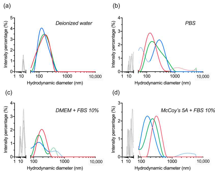
Figure 7. Evaluation of colloidal stability of lyophilized dBSA-UCNP-NOBF 4 in different buffers after six months of lyophilization and mixed by vortexing only, based on the results of three repeated size measurements (shown in blue, red, and green) by DLS: (a) in deionized water; (b) in PBS; (c) in DMEM cell culture medium supplemented with 10% FBS; (d) in McCoy's 5A cell culture medium supplemented with 10% FBS. Gray and/or dotted lines below 100 nm correspond to the presence of proteins and protein aggregates; dotted lines over 300 nm are aggregates.
