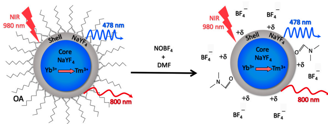
Figure 1. A schematic illustration of upconversion nanoparticles oleic acid (UCNP-OA) core/shell structure and the ligand exchange method converting UCNP-OA into UCNP-NOBF 4 . DMF—dimethylformamide.
