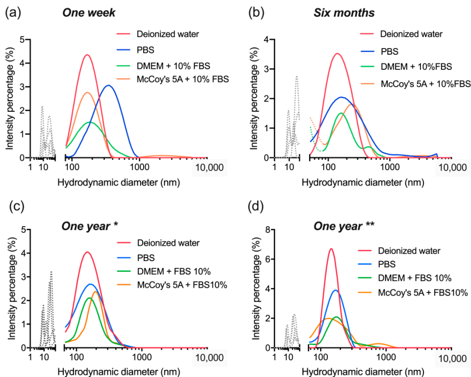
Figure 10. Evaluation of colloidal stability of lyophilized dBSA-UCNP-NOBF 4 in different buffers at all three checkpoints based on the average results of three repeated size measurements by DLS: (a) after one week of lyophilization; (b) after six months; (c,d) after one year. * before ultrasonication, ** after ultrasonication; gray and/or dotted lines below 100 nm correspond to the presence of proteins and protein aggregates.
