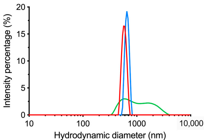
Figure 4. Hydrodynamic diameter of dBSA-UCNP-NOBF 4 after using centrifugation. dBSA-UCNP-NOBF 4 were measured by DLS following the incubation of UCNPs-NOBF 4 (0.25 mg/mL) with dBSA (concentration over 50 \mu M) and centrifuged at 10,000 \times g for 7 min. DLS three repeated size measurements are shown in blue, red, and green.
