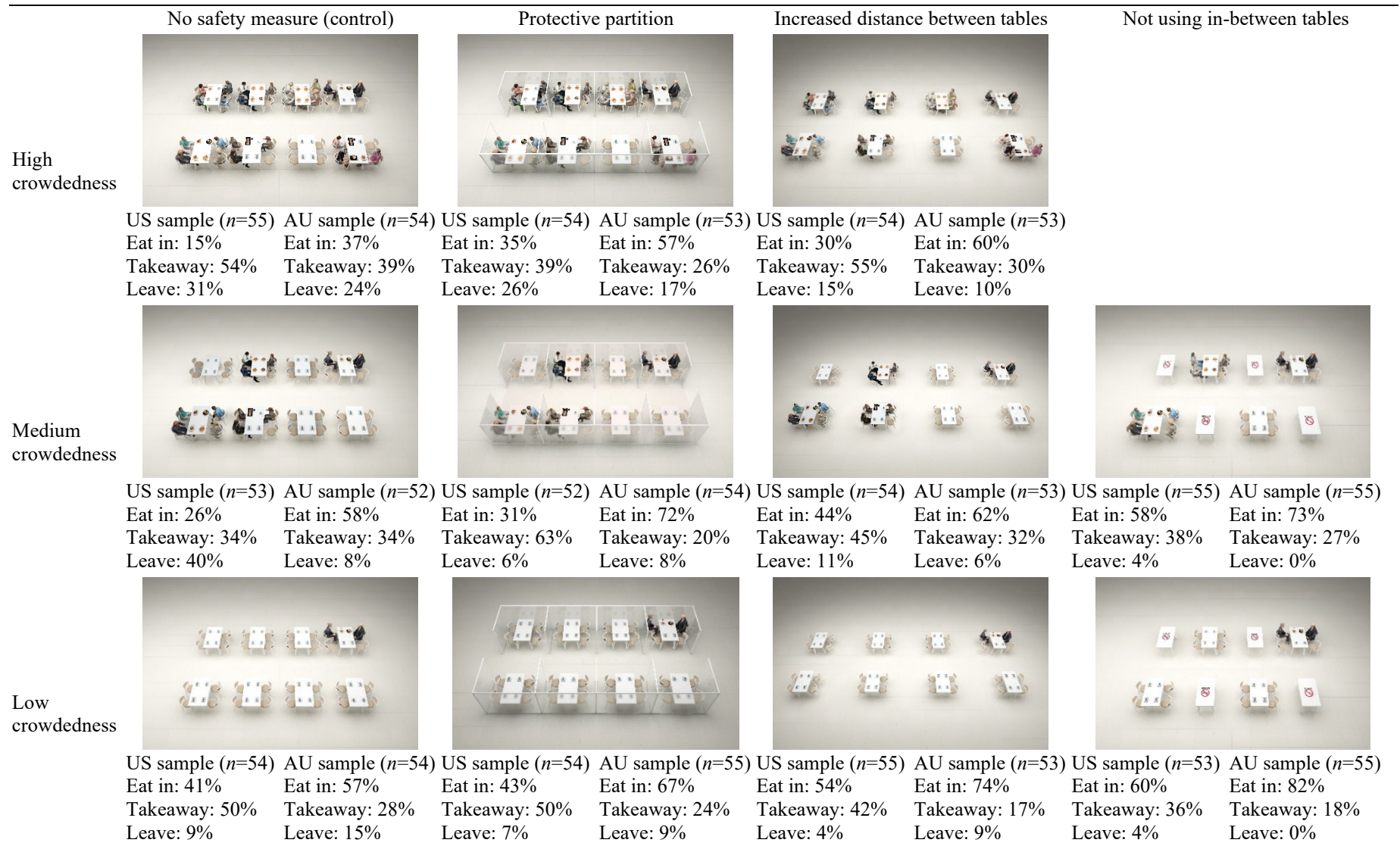
Fig. 2. Choice shares across conditions
