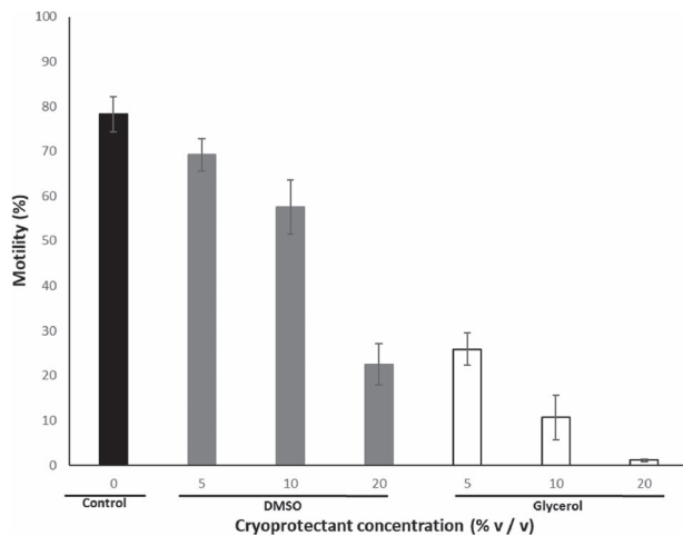
Figure 2: The effect of cryoprotectant type and concentration on percent sperm motility in unfrozen samples incubated for 5 hours at room temperature ( \sim 25°C). The data are presented as raw mean percentage \pm 1 standard error of the mean.
