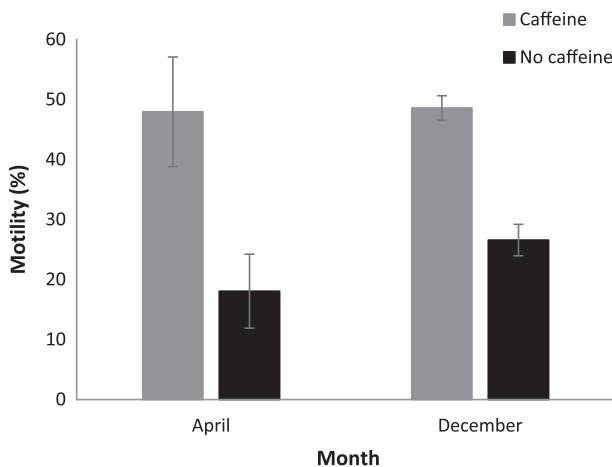
Figure 5: Comparison of post-thaw sperm motility between animals captured during April ( n = 2 ) and December ( n = 3 ) for samples frozen with 10% v/v DMSO, with or without the presence of caffeine. Data are presented as raw means \pm 1 standard error of the mean (derived from 12 repetitions per animal).
