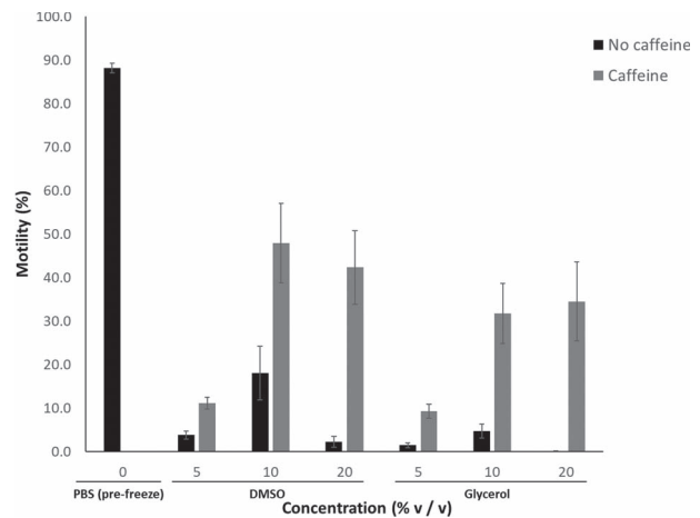
Figure 4: The effect of cryoprotectant type and concentration during cryopreservation and the addition of 10 mM caffeine post-thaw on percent sperm motility assessed after thawing of samples. Data are presented as raw means \pm 1 standard error of the mean.
