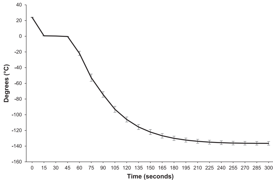
Figure 1: Cooling rate of water suspended 5 cm above LN 2 , immersed in vapour and cooled over 5 minutes. The data are presented as raw means \pm 1 standard error of the mean (n = 4 repetitions).
