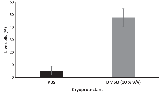
Figure 6: Comparison between the percentage of live cells following sperm cryopreservation ( n = 4 ) with 10% v/v DMSO. Data are presented as raw means \pm 1 standard error of the mean.
