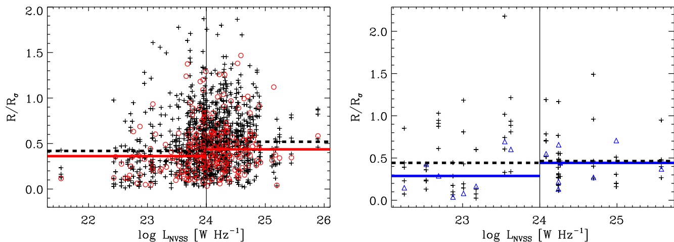
Figure 8. The normalized radial distance of radio galaxies from the group centre as a function of radio luminosity. Left: LERGs (red circles) and their controls (black crosses); right: HERGs (blue triangles) and their controls (black crosses). The radial distance is normalized by the radius containing 68 per cent of the group members, R_\sigma for each group. The horizontal lines indicate the median value of the radial distribution for radio galaxies (solid lines) and their control samples (dashed black lines) in the two different radio luminosity bins.
